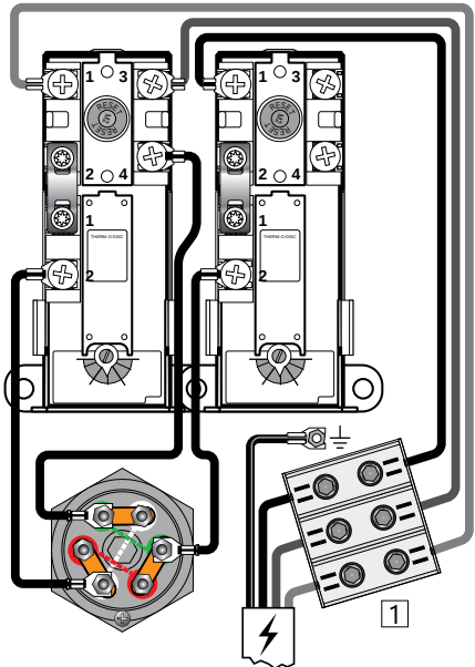
Electrical connection, diagram OPTIONAL
