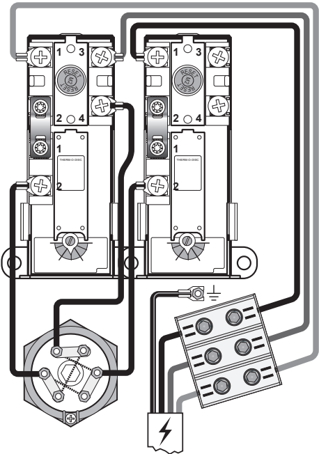
Wiring diagram - 3x230V Standard connection for lower cylinder OGC 360 supplied with two 7.5 kW junction boxes
